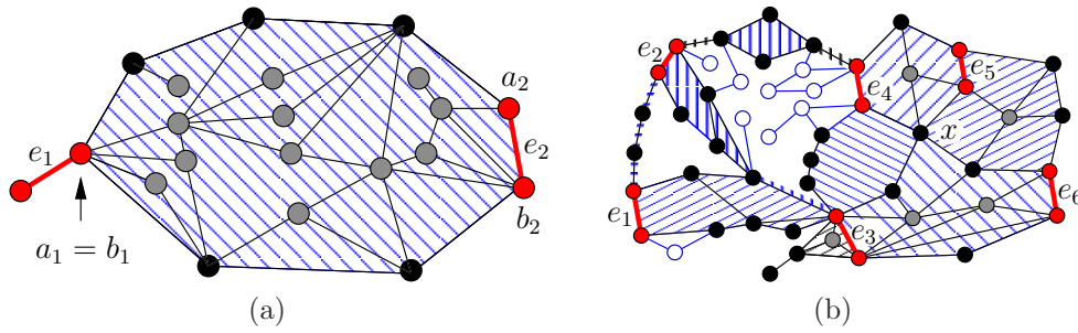
Figure 8.2: (a) Example of region R(e_1, e_2) between two edges e_1, e_2 \in M . Note that e_1 is not part of R , but only its endpoint a_1 = b_1 . The black vertices are the boundary vertices, and the gray vertices in the hatched area are the vertices strictly inside of R . (b) An example of an M -region decomposition: white vertices lie outside of regions and each region is hatched with a different pattern.
